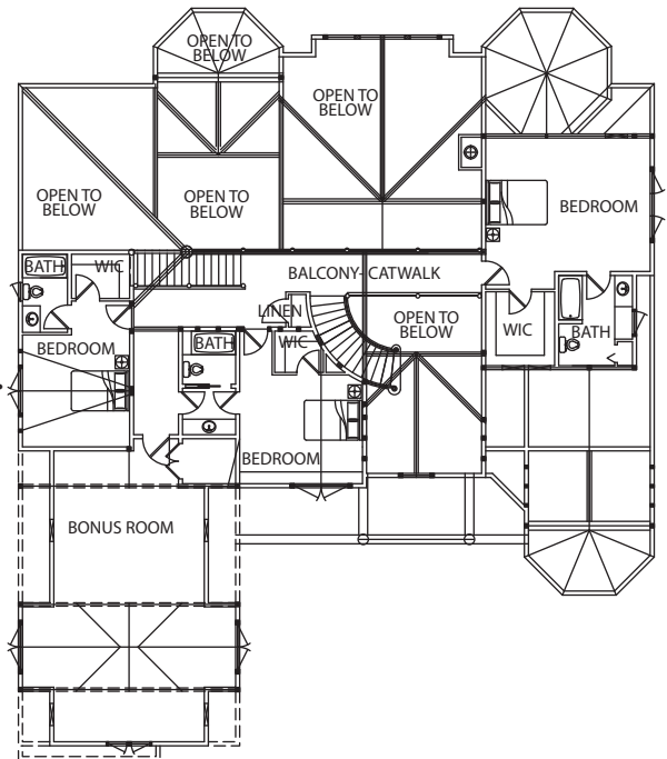
SECOND FLOOR: 1,416 SQ. FT.
