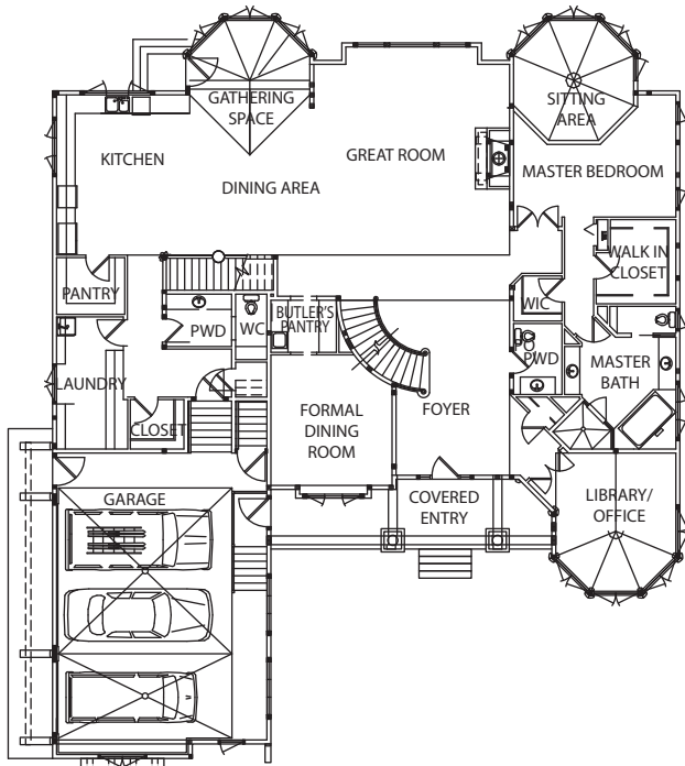
FIRST FLOOR: 3,635 SQ. FT.
