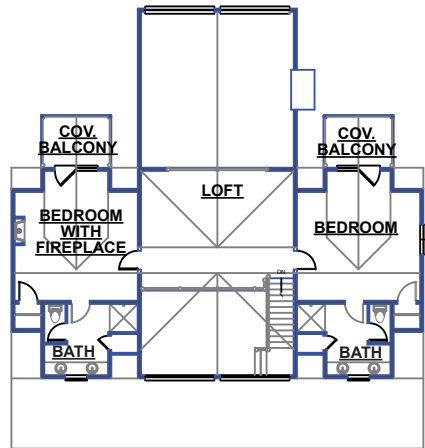
SECOND FLOOR PLAN 1,488 S.F.
