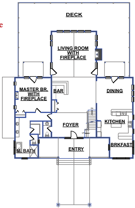
FIRST FLOOR PLAN 2,514 S.F.
