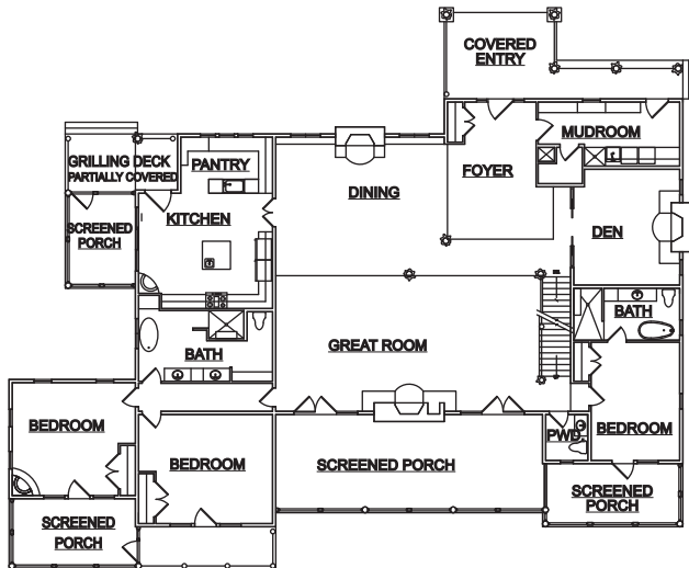
FIRST FLOOR: 3,988 SQ. FT. PLUS SCREENED PORCHES: 976 S.F.
